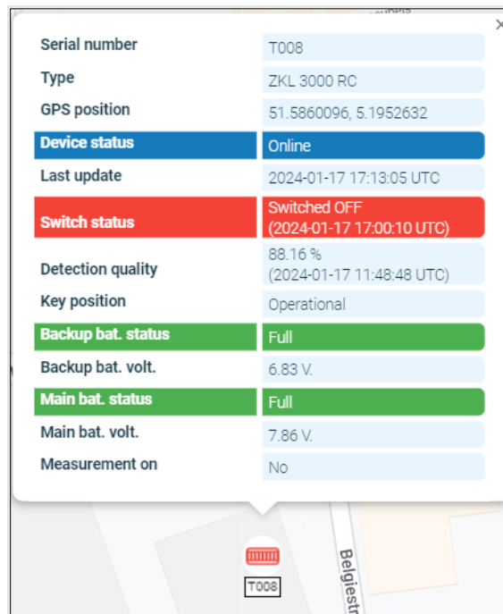
Figure 110 Real-time status ZKL 3000 RC
