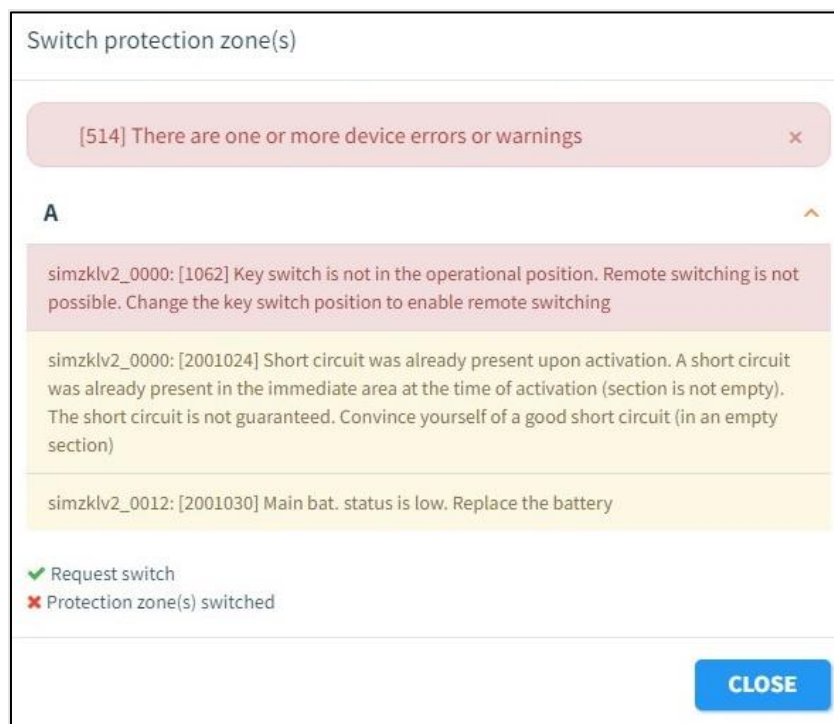
Figure 75 Device error/warning message
