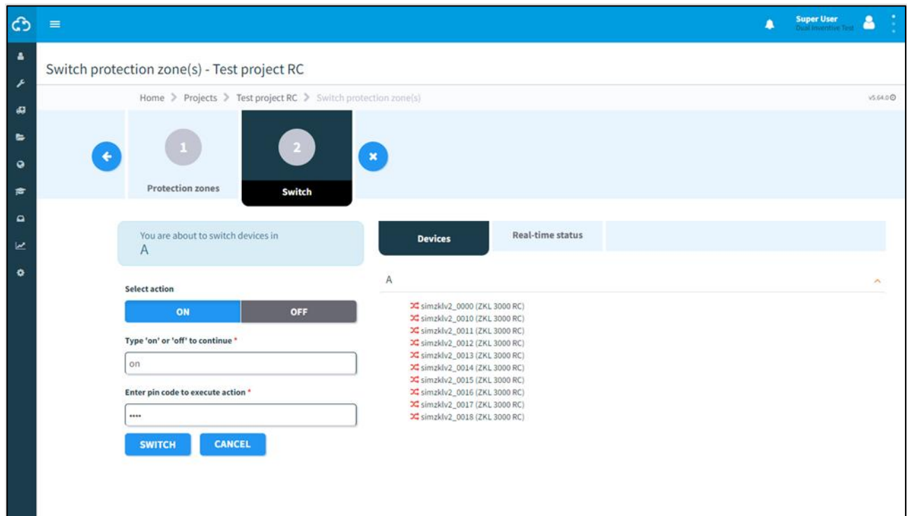
Figure 72 Switch devices page
